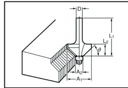
Ball bearing chamfering bit
