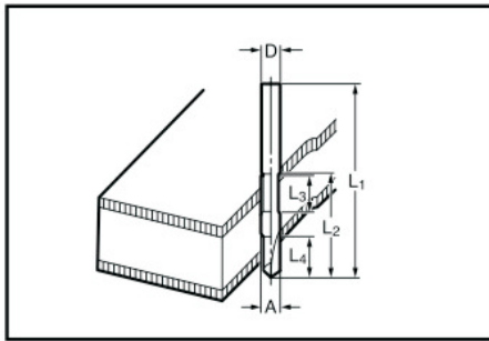
Drill point double flush trimming bit
