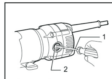
► 1. Screwdriver 2. Brush holder cap
