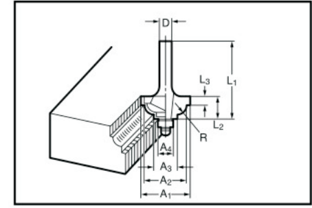
Ball bearing cove beading bit
