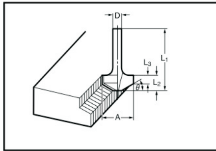
Chamfering bit
