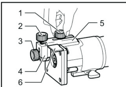
► 1. Clamp screw (A) 2. Adjusting screw 3. Clamp screw (B) 4. Trimmer guide 5. Guide holder 6. Chip deflector
