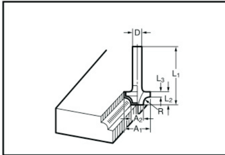
Corner rounding bit
