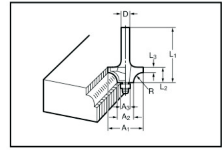
Ball bearing beading bit
