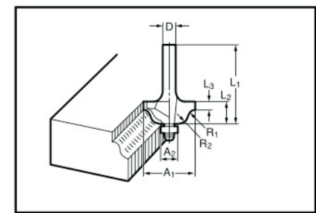
Ball bearing roman ogee bit
