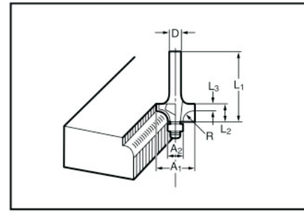
Ball bearing corner rounding bit
